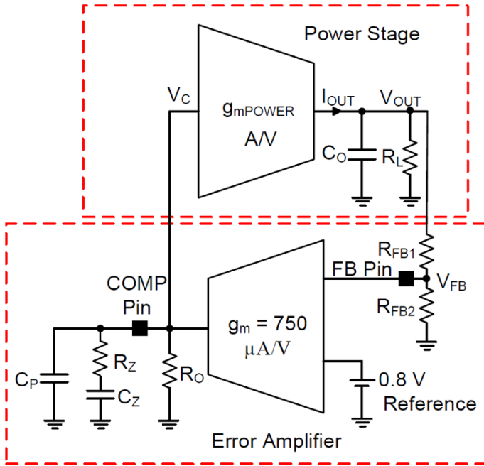
Figure 10: Power Stage and Error Amplifier
