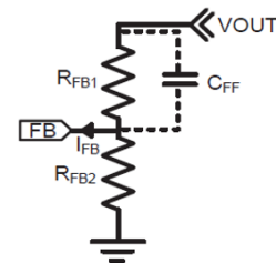
Figure 11: Feedback Divider with Feedforward Capacitor
