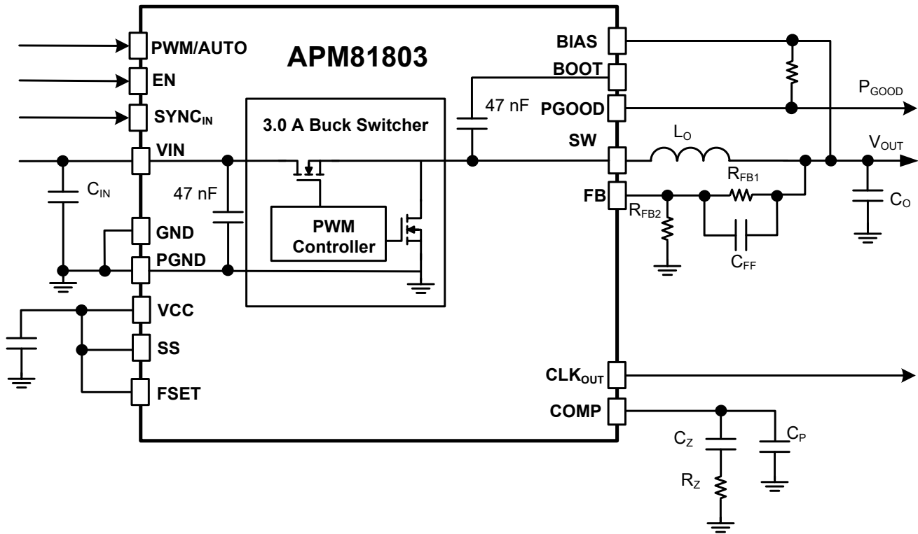
Figure 12: Applications Schematic showing component locations
