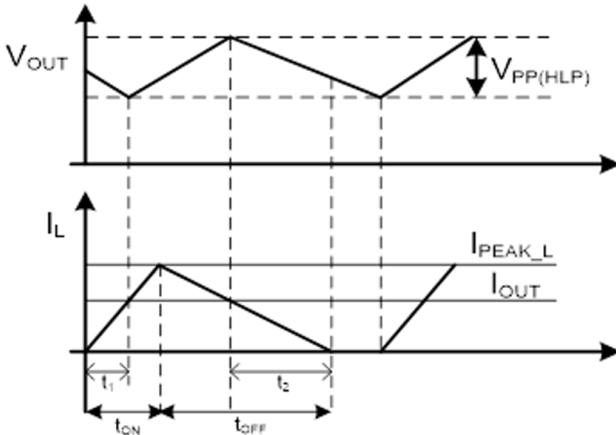
Figure 8: Output Voltage Ripple in LP Mode
