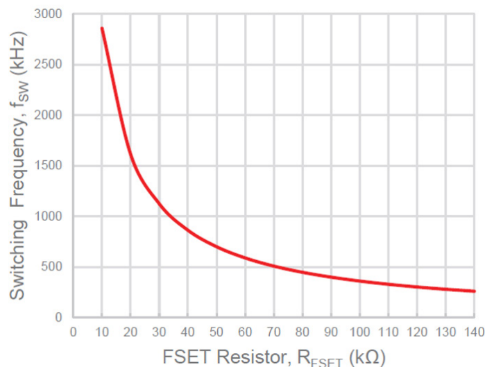
Figure 6: PWM Switching Frequency vs. R_{FSET}
